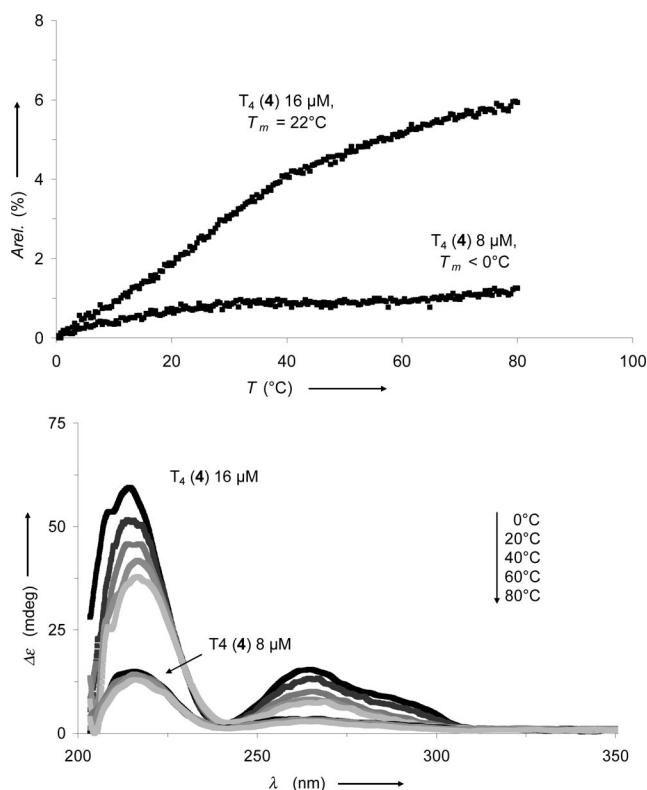
Figure 8. Temperature-dependent UV melting curve and CD spectra of self-aggregating thymynyl \beta -peptide 4 ( 8\ \mu\text{M} and 16\ \mu\text{M} , 10\ \text{mM} Tris·HCl buffer, pH 7.5).
