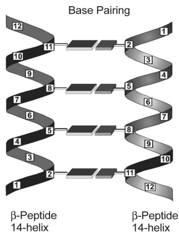
Figure 1. Model of antiparallel base pairing \beta -peptide helices uniformly functionalized with nucleobases in every third position.
