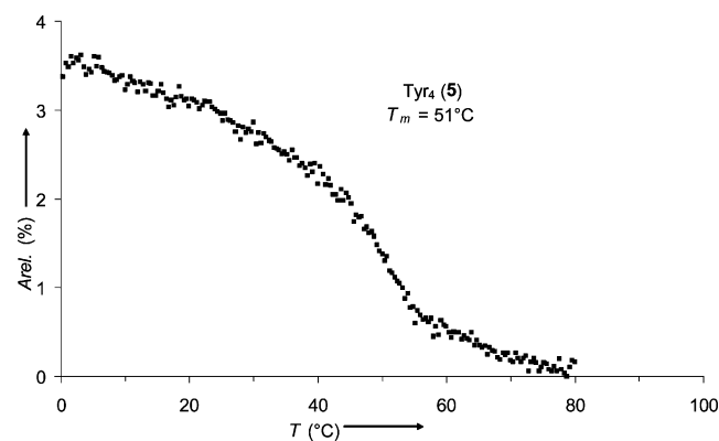
Figure 5. UV melting curve of oligomer 5 (8 \mu mol, 10 mM Tris-HCl buffer at pH 7.5).
