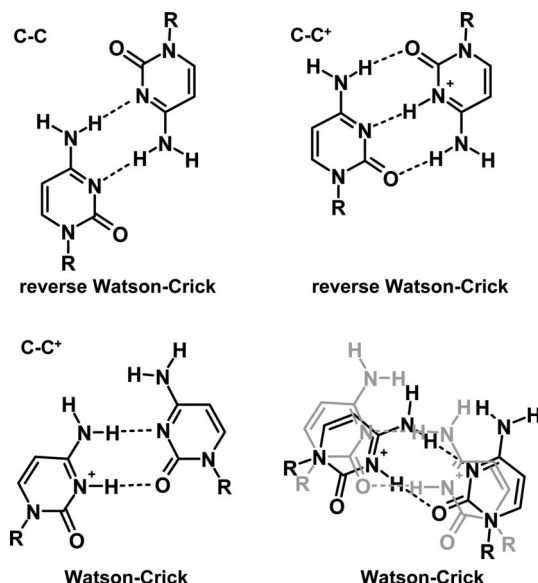
Figure 7. C–C base pairing: semi-protonation at pH 4.5 allows formation of a tridentate reverse Watson–Crick mode next to a two-dentate Watson–Crick base pair.
