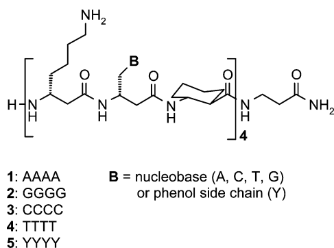
Figure 2. \beta -Peptides 1–5 uniformly functionalized with nucleobases (A, G, C, T) or with a tyrosine (Y) side chain.
