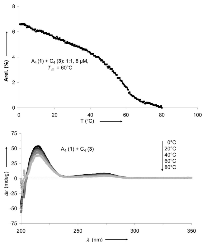
Figure 12. UV melting curve and CD spectra of an equimolar mixture of oligomers 1 and 3 ( 4\ \mu\text{M} each, 10 mM Tris-HCl buffer, pH 7.5).
